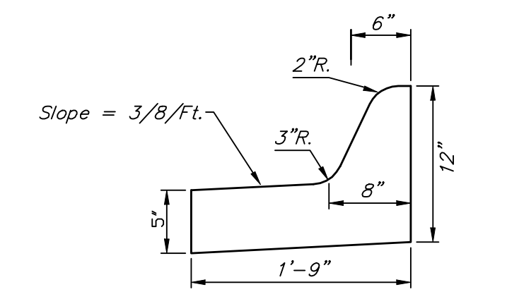
Medial Curb Detail (Low Edge) Not to Scale
