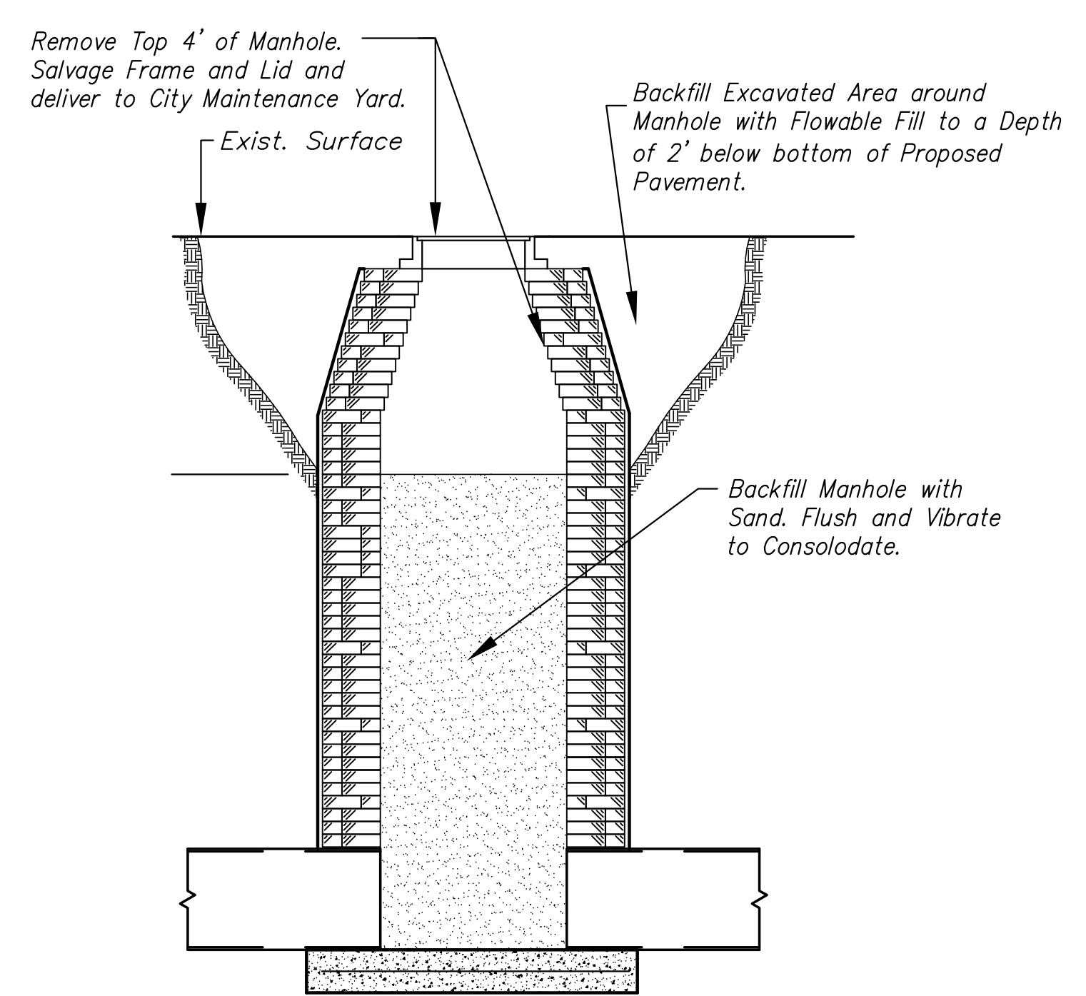
MANHOLE ABANDON DETAIL
