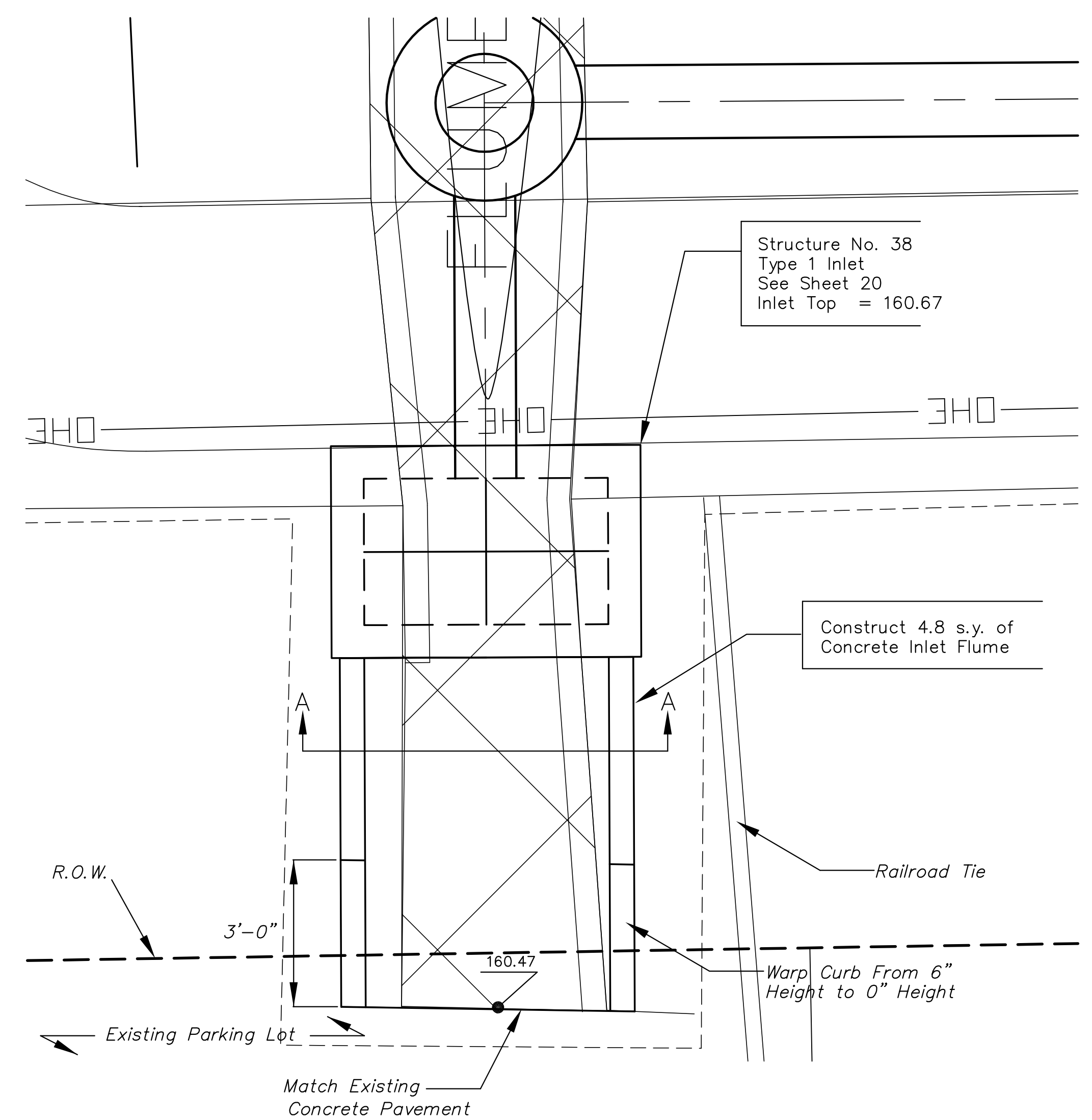
INLET FLUME DETAIL (Sta. 40+50.95)
