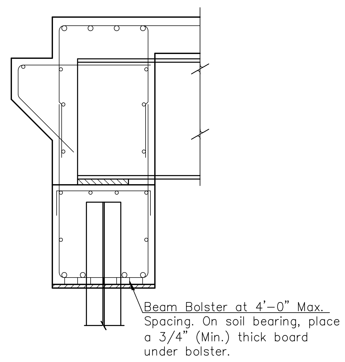
ABUTMENT
