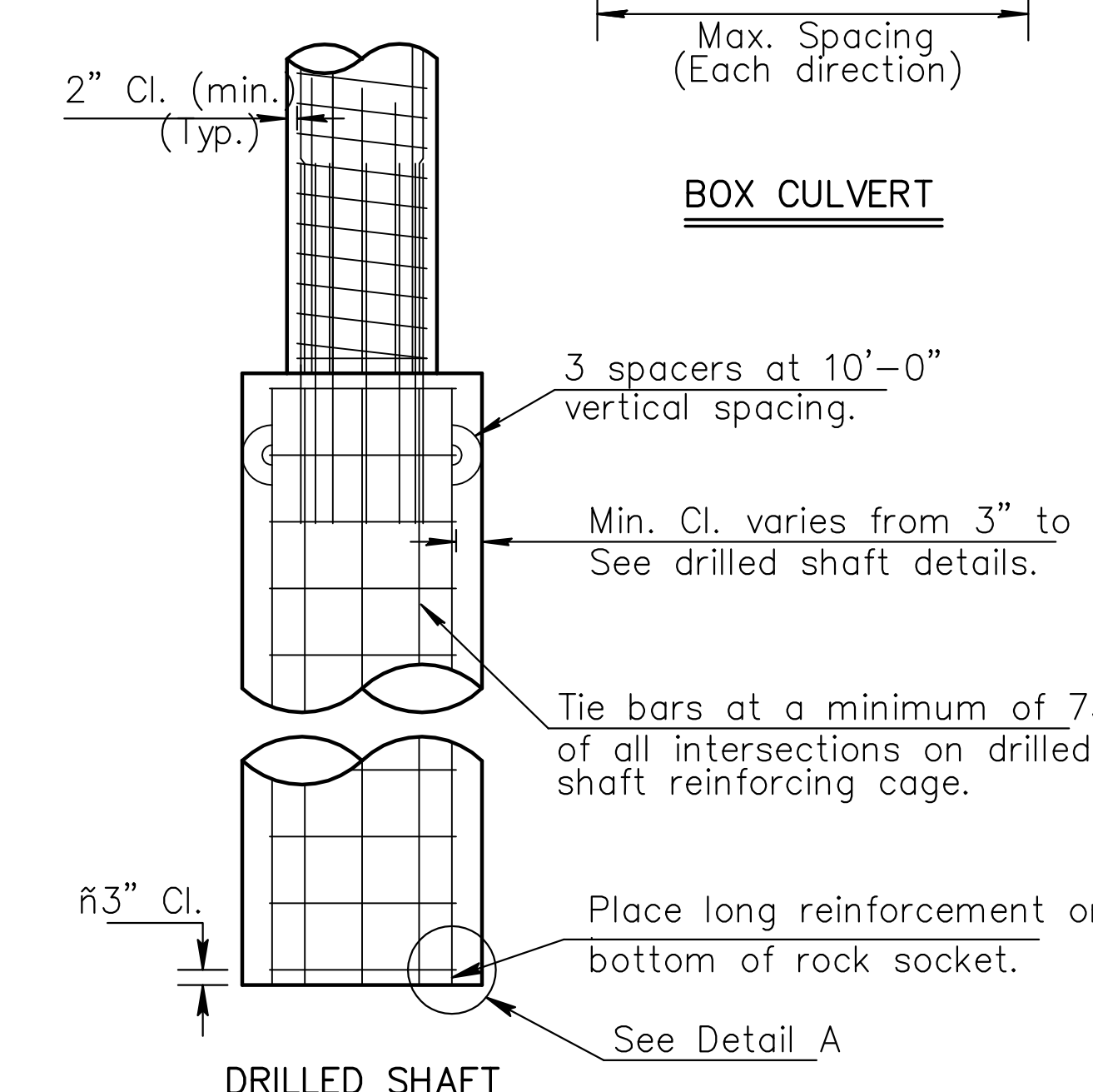
DRILLED SHAFT
