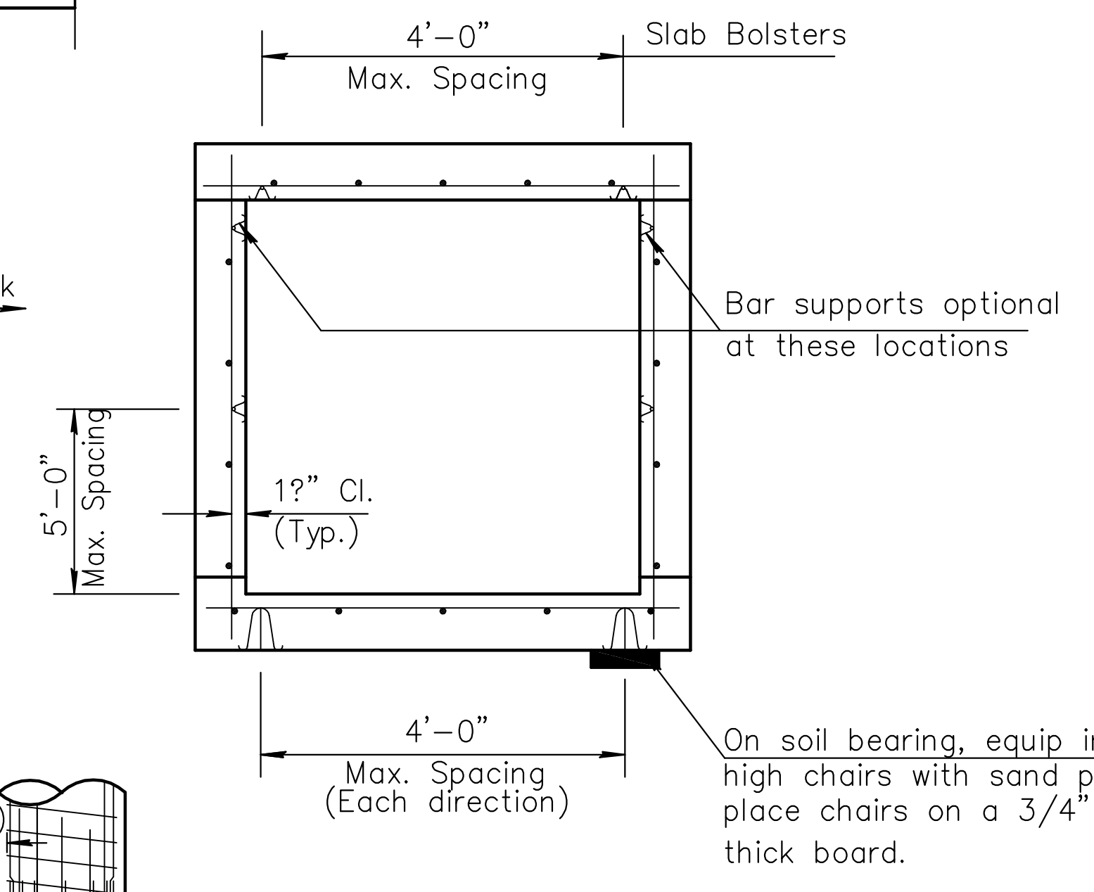
BOX CULVERT
