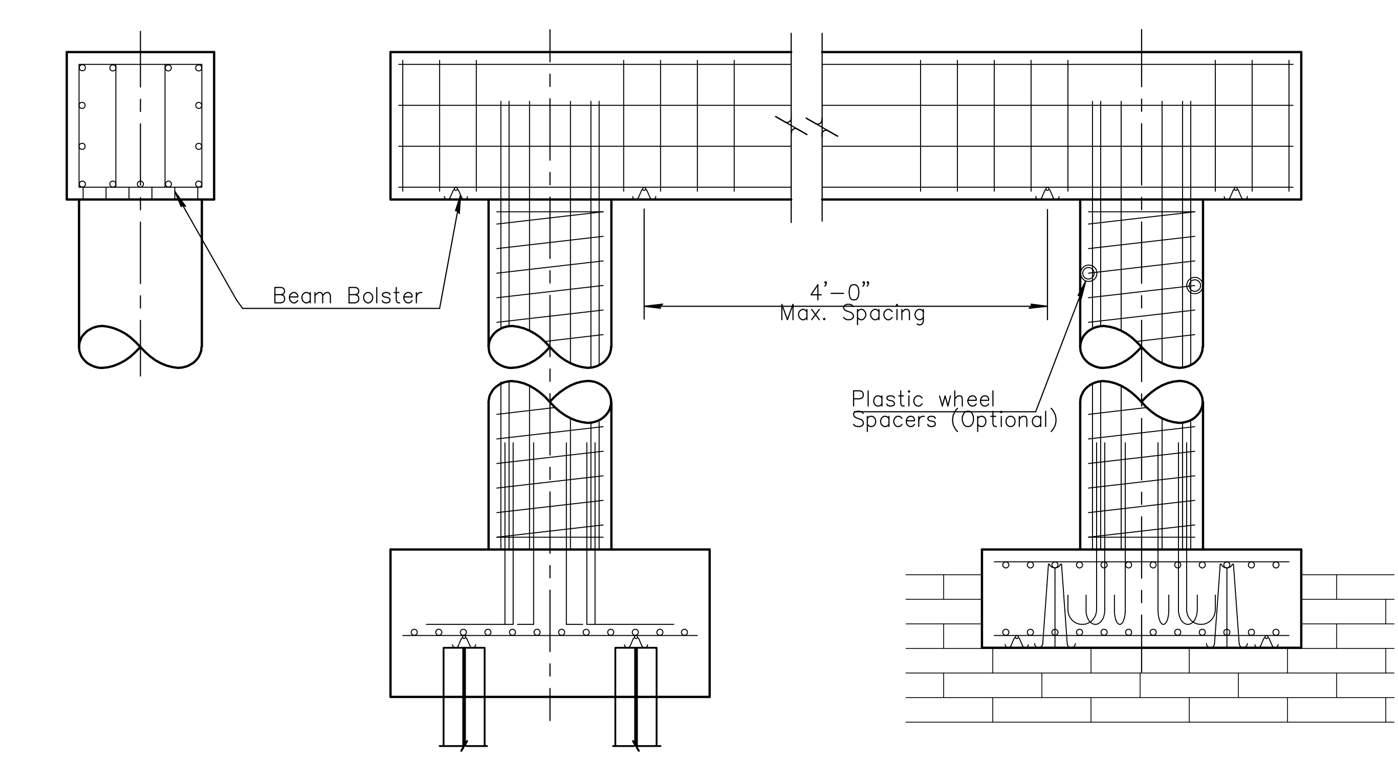
PIER
