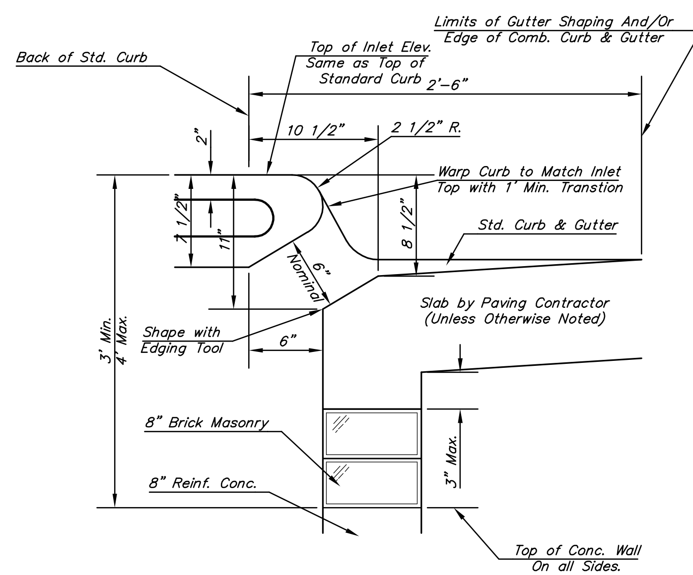
SECTION B-B
