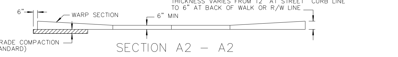
FULL RAMP DRIVES (P = 4.0' & 6.5')
