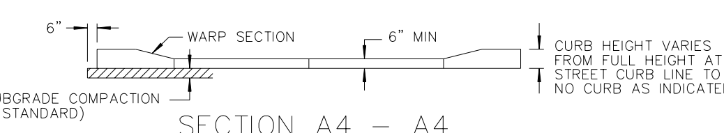
FULL RAMP DRIVES (P = 7.0' & 8.5')
