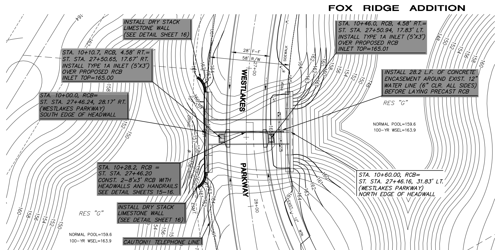
FOX RIDGE ADDITION PLAN RCB
