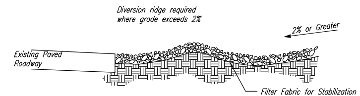
SECTION C-C
