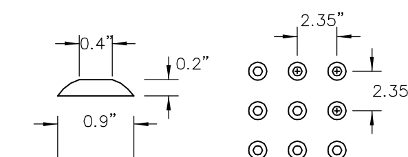
DOME DETAIL
