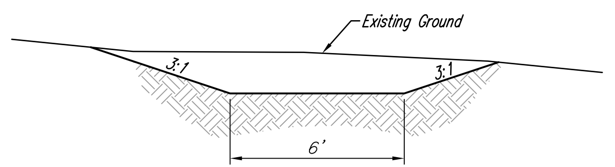
DITCH SECTION
