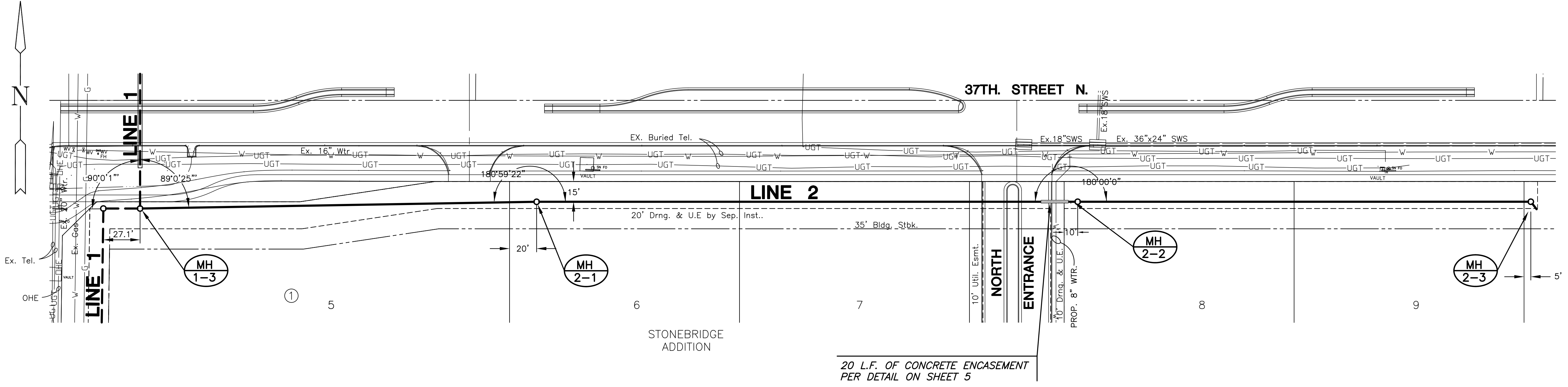
PLAN LINE 2
