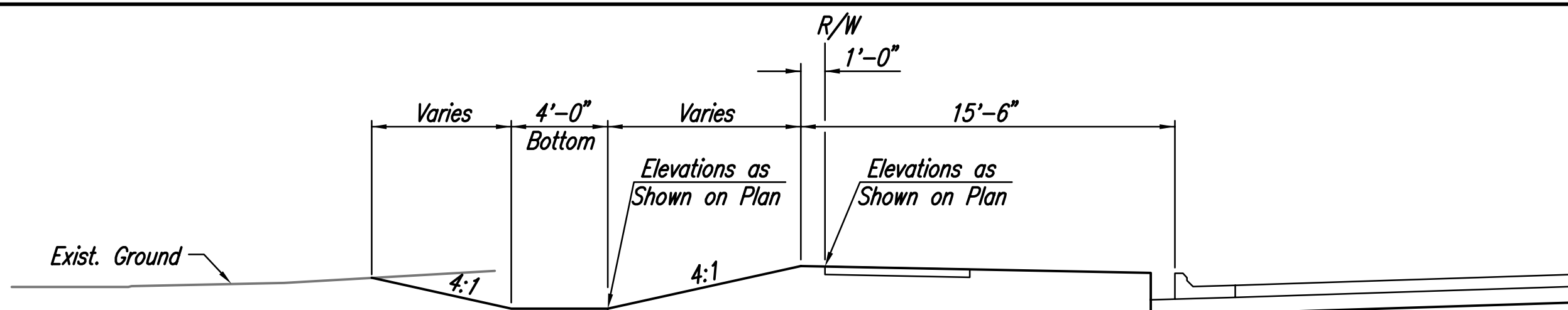
SECTION B-B Sta. 13+00± to Sta. 17+75± See Cross Sections No V.C.
