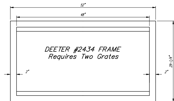
Double 24" x 24" Frame Detail
