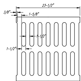
DEETER #2433 GRATE
