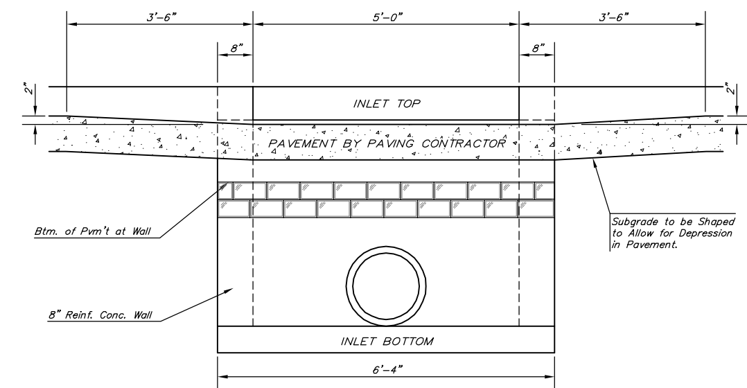
SECTION E-E
