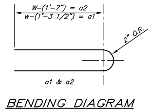
BENDING DIAGRAM
