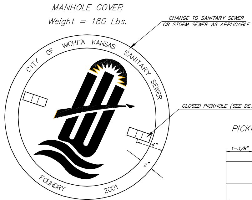
TOP VIEW
