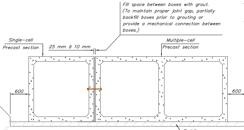
TYPICAL INSTALLATION DETAILS (Example Only)
