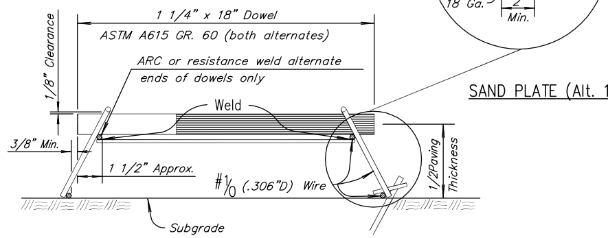
SEC. B-B
