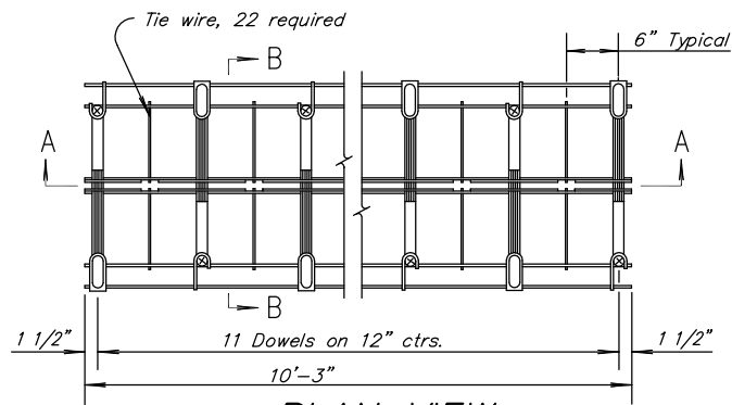
PLAN VIEW
