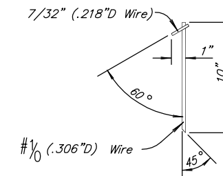
STAKE DETAIL
