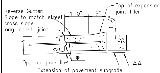
TYPICAL SECTION
