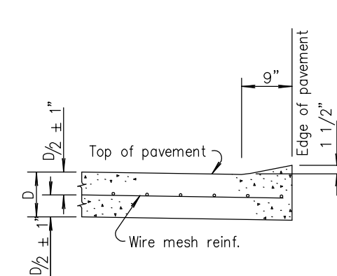
TYPICAL SECTION
