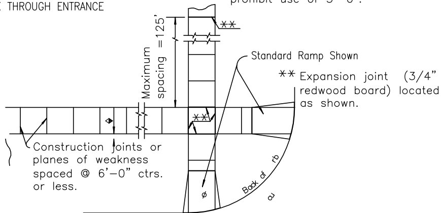
TYPICAL PLAN SIDEWALK
