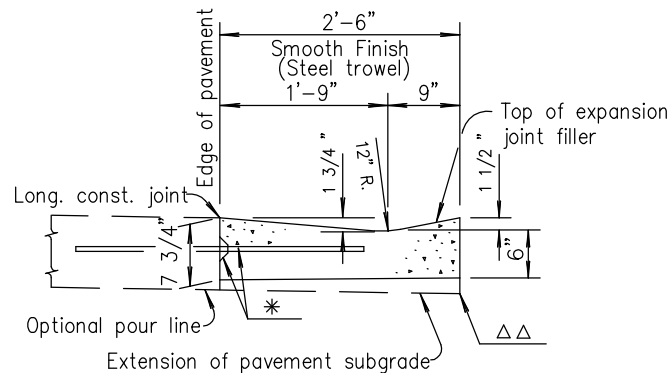
TYPICAL SECTION
