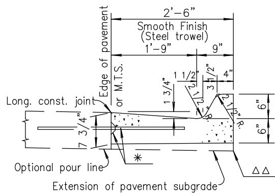
TYPICAL SECTION
