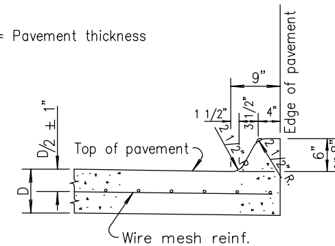
TYPICAL SECTION
