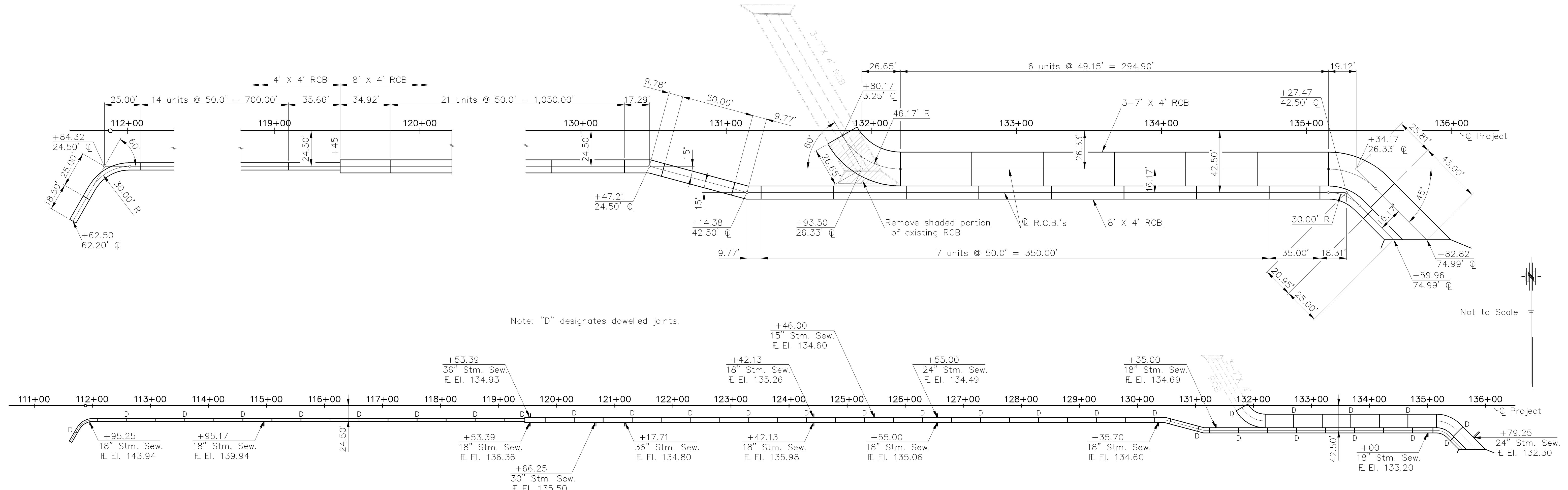
PLAN
