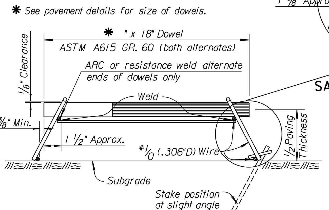
SEC. B-B
