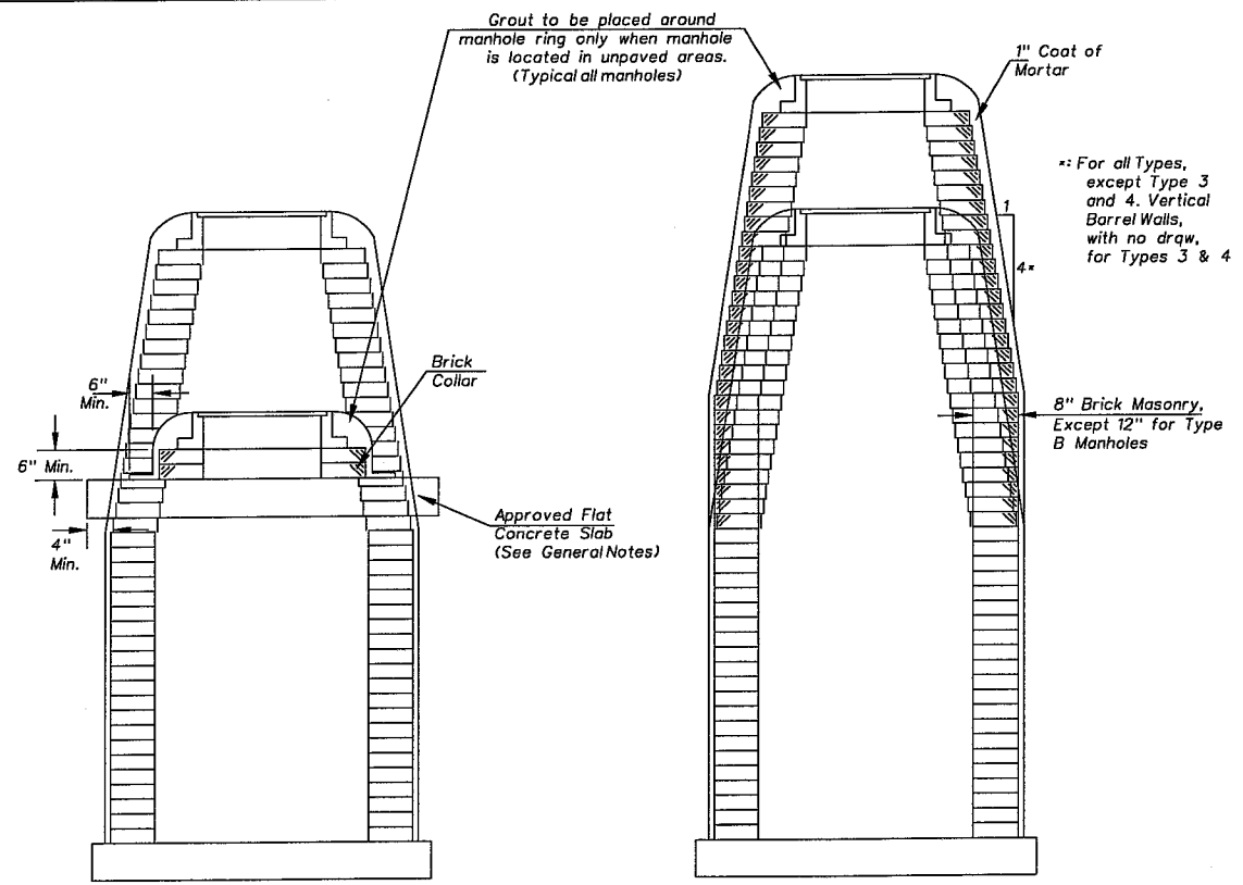
DOWNWARD ADJUSTMENT (GREATER THAN 12")
