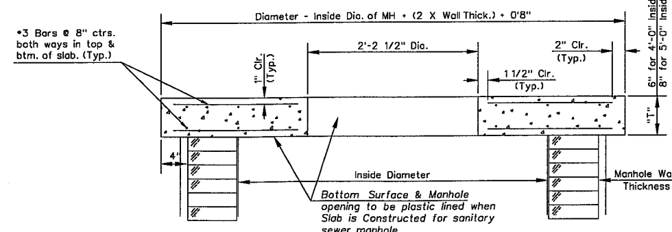
SECTION A-A FLAT CONCRETE SLAB DETAILS
