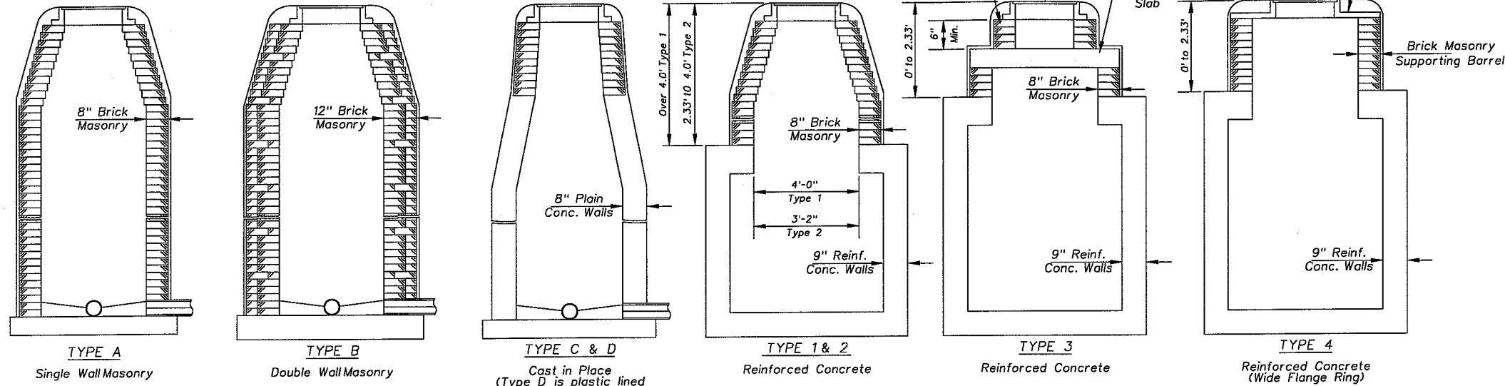
DEFINITION SKETCHES - CITY OF WICHITA STANDARD MANHOLES
