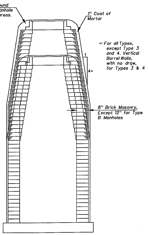
UPWARD ADJUSTMENT (GREATER THAN 12")
