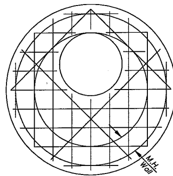
* PLAN ALTERNATE OPENING LOCATION
