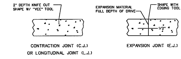
CONTRACTION JOINT (C.J.) OR LONGITUDINAL JOINT (L.J.)
