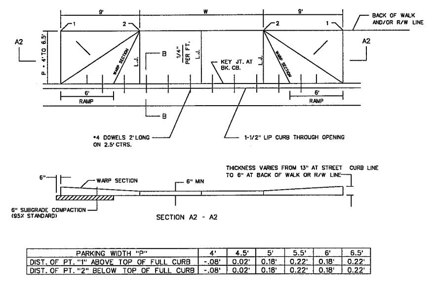
FULL RAMP DRIVE (P = 4.0' TO 6.5')
