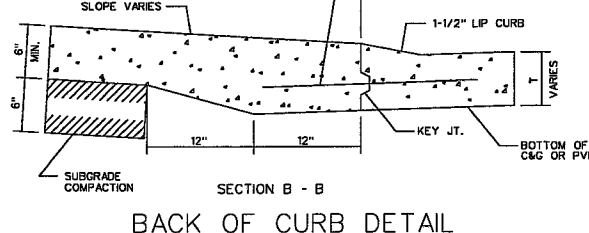
BACK OF CURB DETAIL
