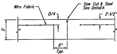
CONTRACTION JOINT DETAIL (C.J.)
