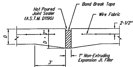
EXPANSION JOINT
