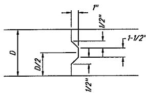
KEYWAY DETAIL
