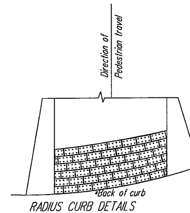
RADIUS CURB DETAILS
