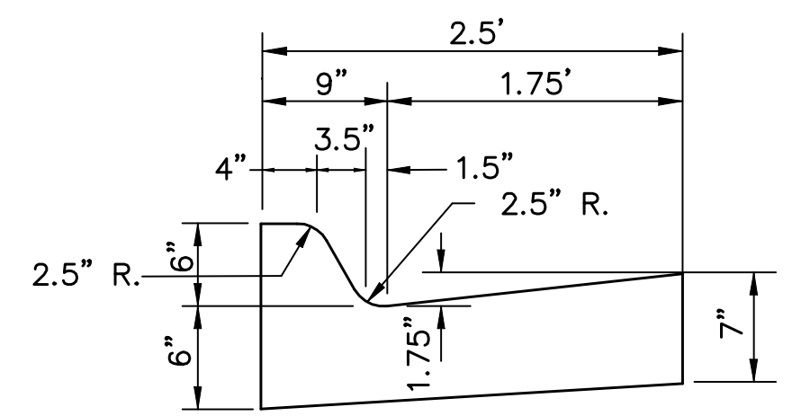
COMBINED CURB & GUTTER TYPE 1
