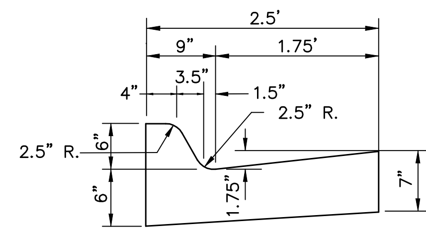
COMBINED CURB & GUTTER TYPE 1
