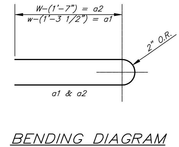
BENDING DIAGRAM
