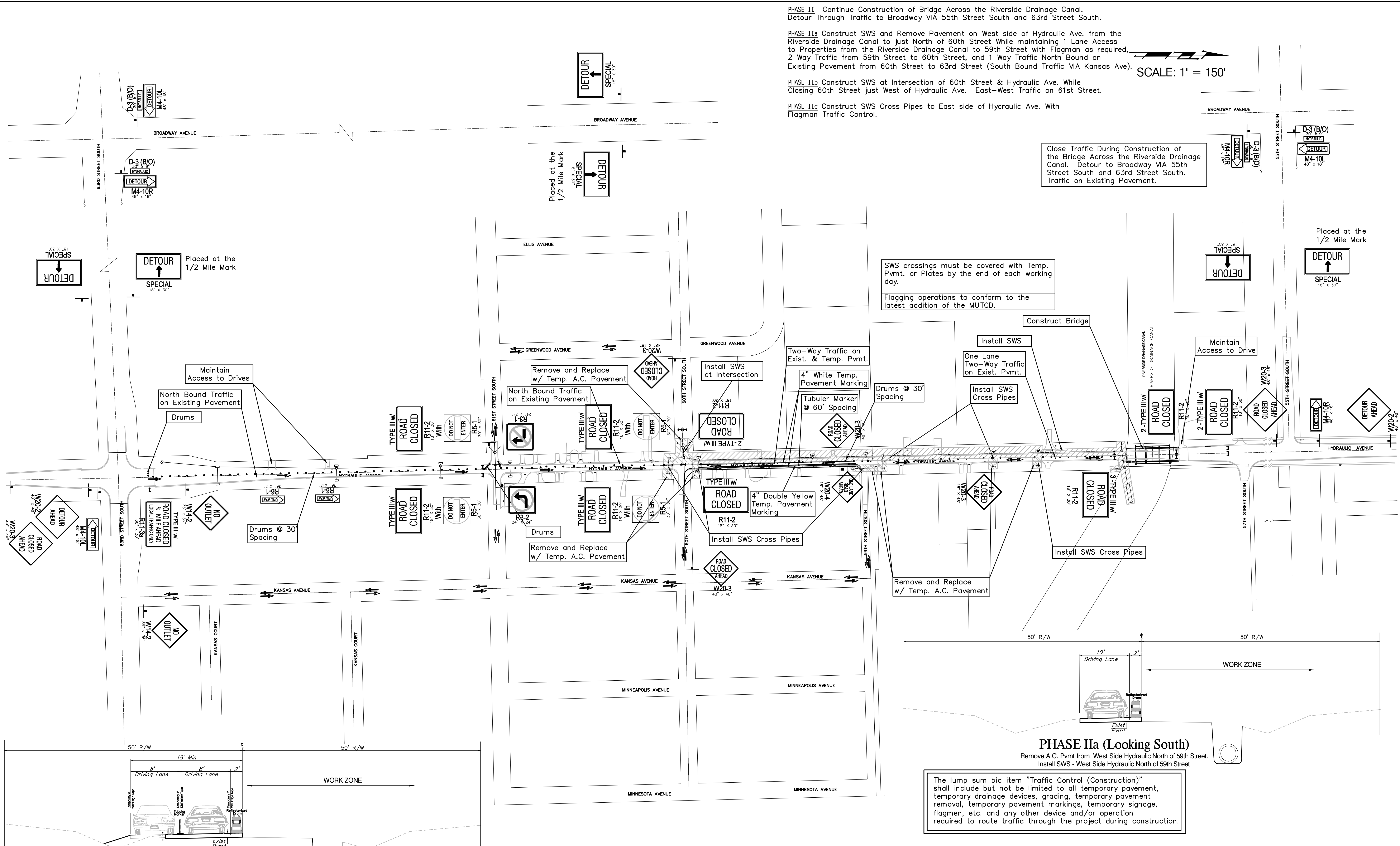
PHASE IIa (Looking South) Remove A.C. Pvmt from West Side Hydraulic 59th Street to 60th Street Install SWS - West Side Hydraulic 59th Street to 60th Street
