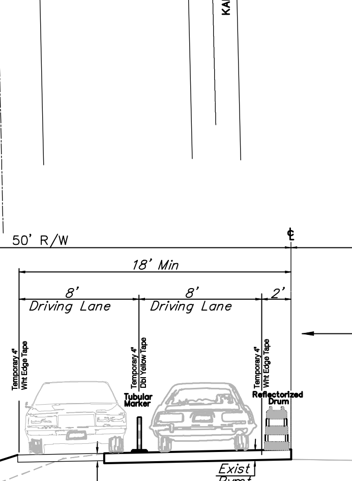
PHASE IIa (Looking South) Remove A.C. Pvmt from West Side Hydraulic 59th Street to 60th Street Install SWS - West Side Hydraulic 59th Street to 60th Street
