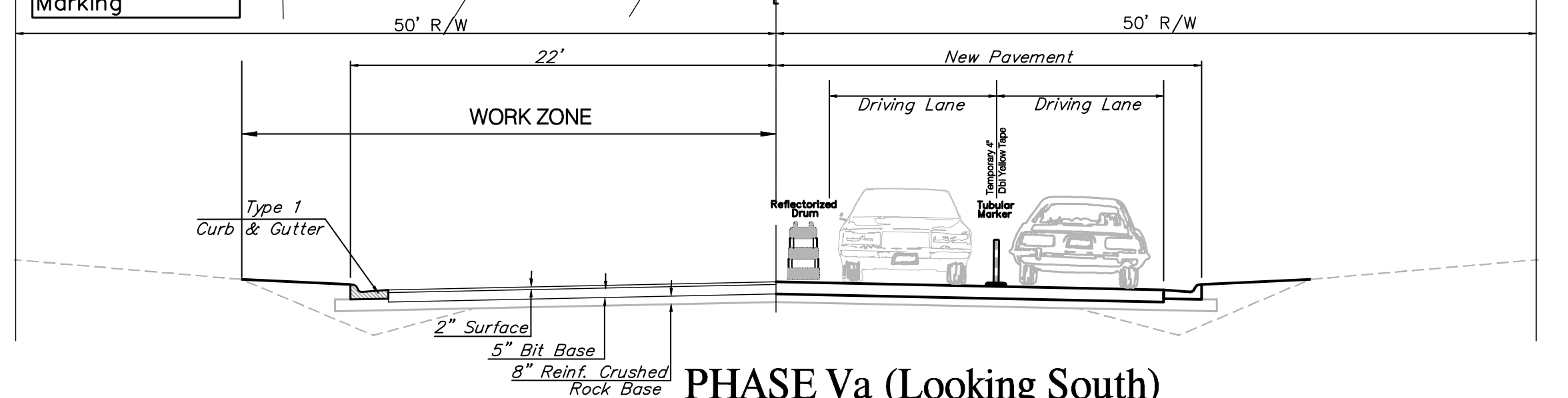
PHASE Va (Looking South) Construct Roadway - East Side Hydraulic, North of 63rd Street to North of 59th Street.
