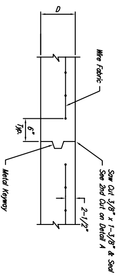
OPTIONAL CONTRACTION JOINT
