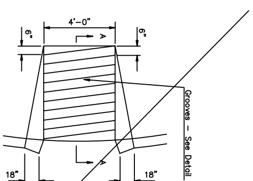
WHEELCHAIR RAMP PLAN VIEW
