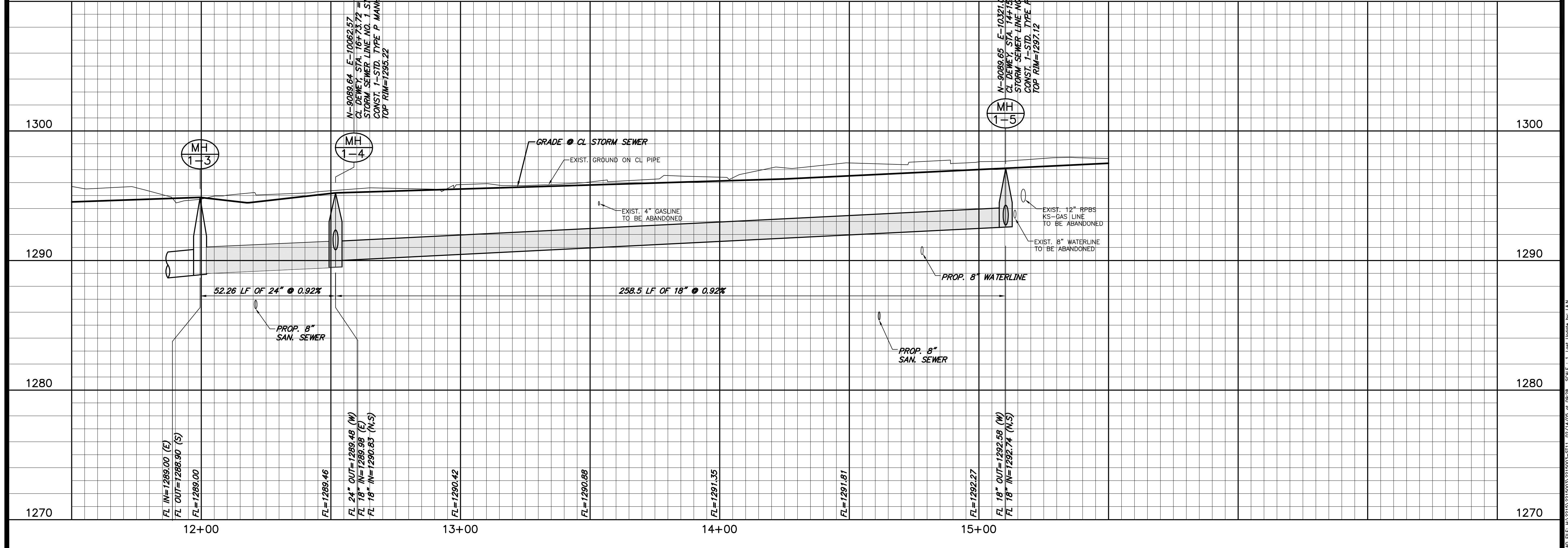
DEWEY STREET STORM SEWER PLAN & PROFILE
