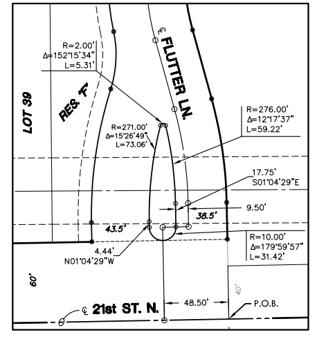
DETAIL RESERVE "A" 1"=50'
