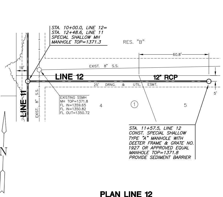
PLAN LINE 12
