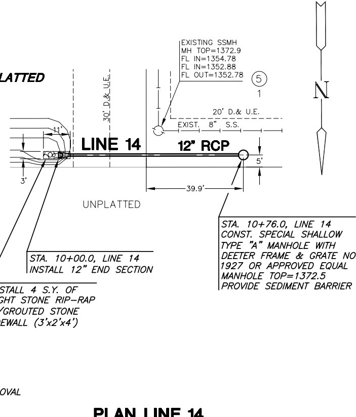
PLAN LINE 14
