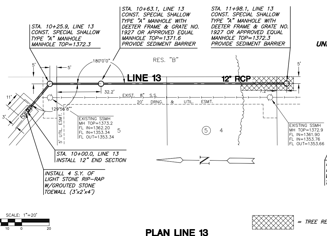
PLAN LINE 13
