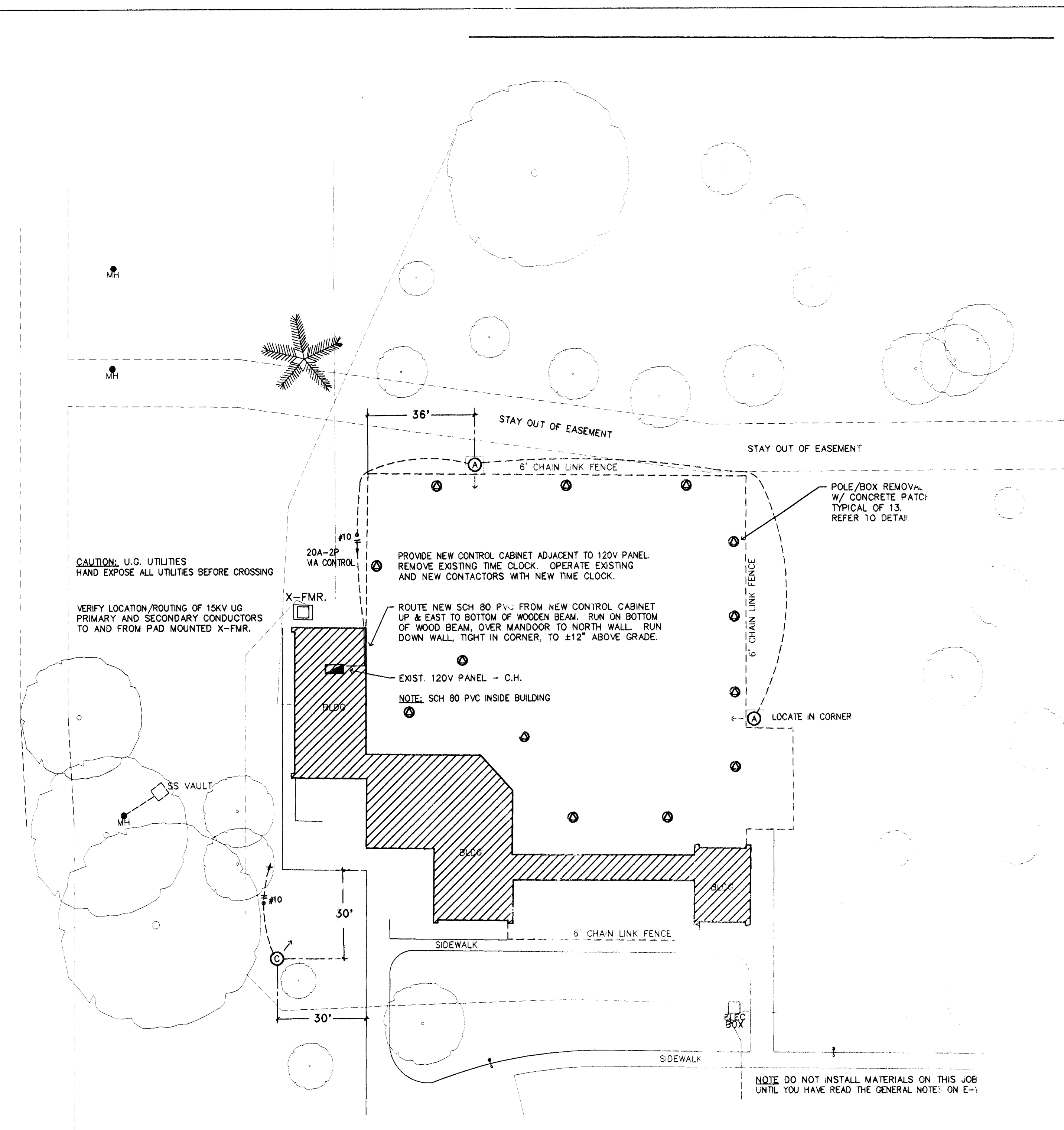
EVERGREEN POOL SITE LIGHTING PLAN
