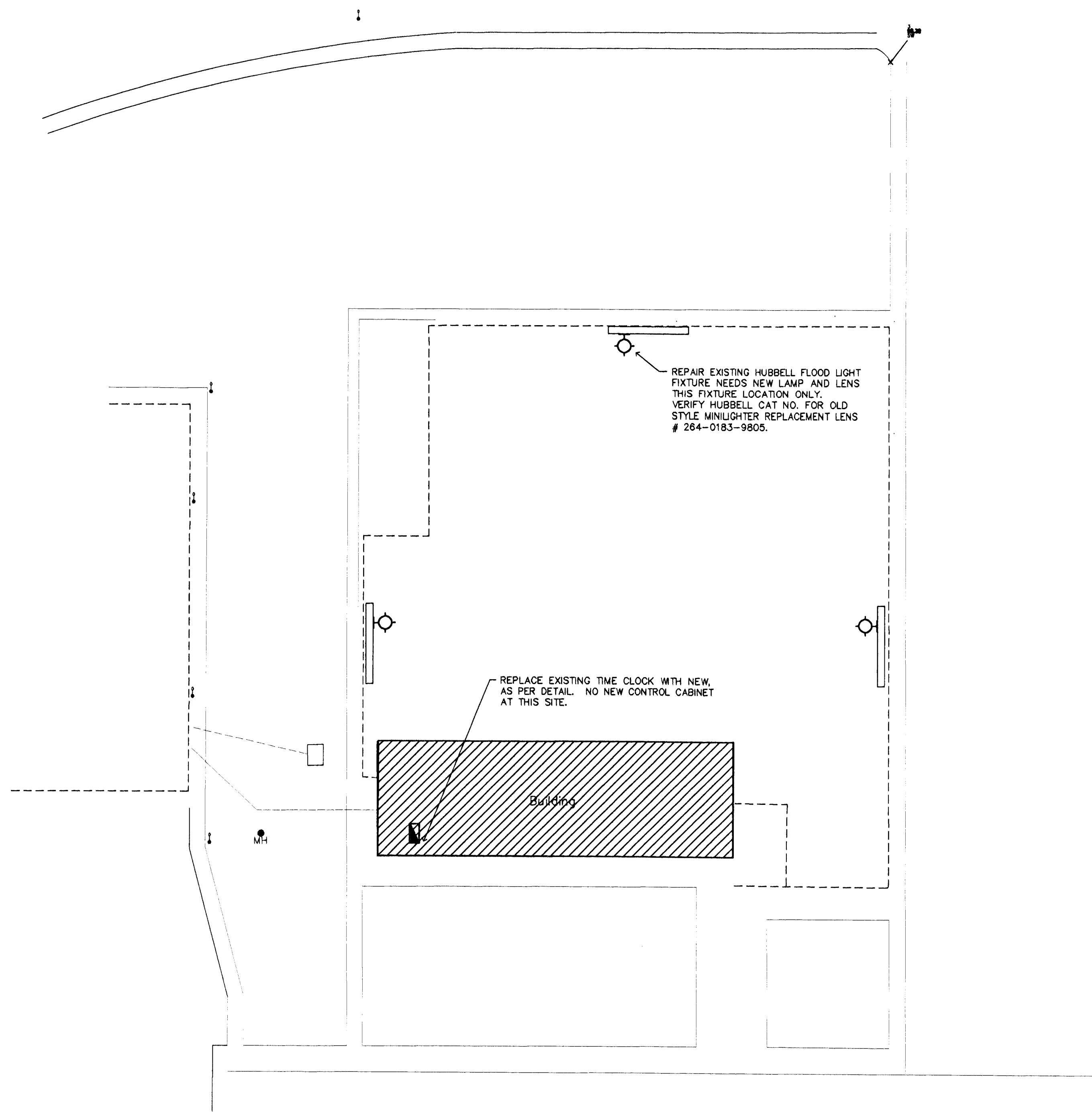
McADAMS SWIMMING POOL SITE LIGHTING PLAN SCALE: 1" = 10'
