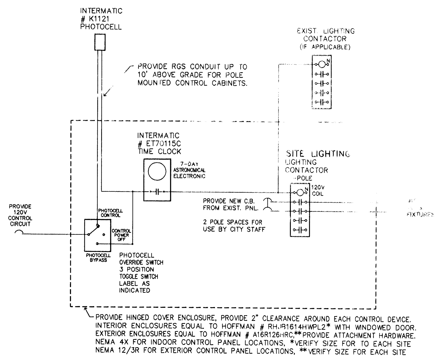
TYPICAL SITE LIGHTING CONTROL
