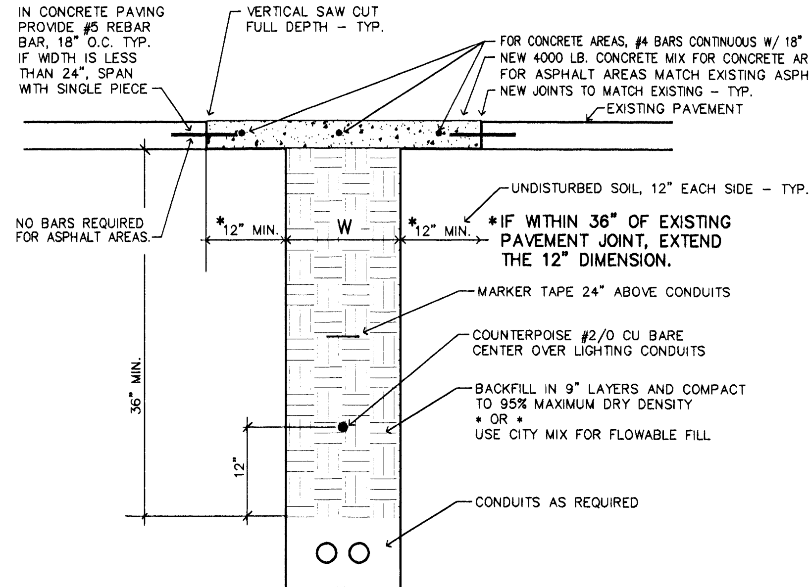
TRENCH BELOW PAVEMENT DETAIL
