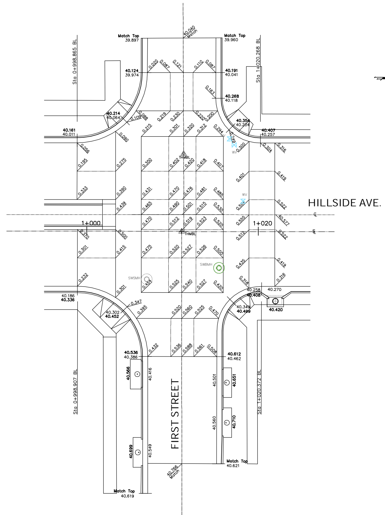
INTERSECTION GRADING PLAN
