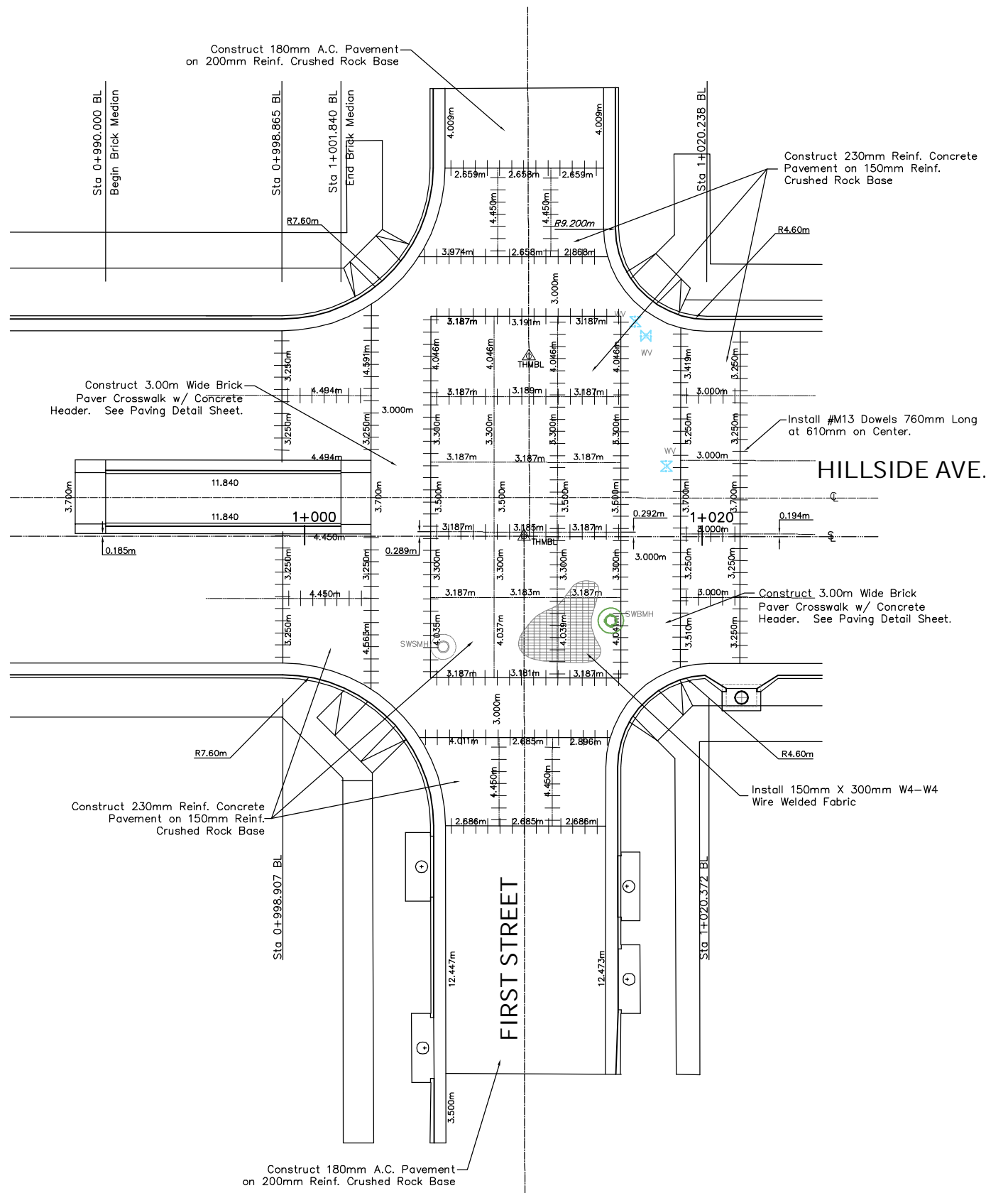
INTERSECTION JOINT PLAN
