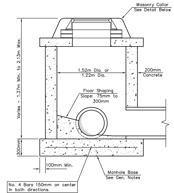
SHALLOW TYPE "C" MANHOLE
