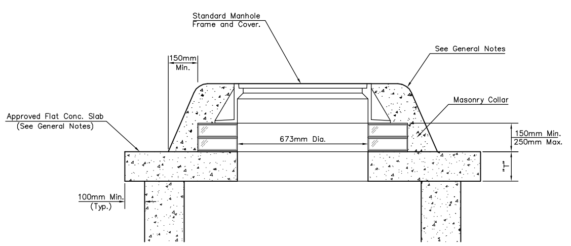
MASONRY COLLAR DETAIL
