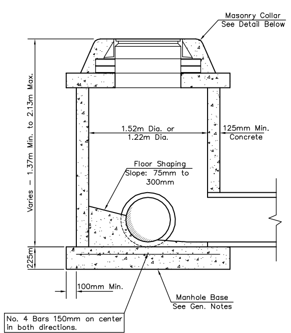
SHALLOW TYPE "P" MANHOLE
