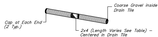
CURB INLET PROTECTION 4" Perforated Pipe w/ Gravel
