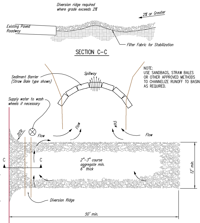
STABILIZED CONSTRUCTION ENTRANCE
