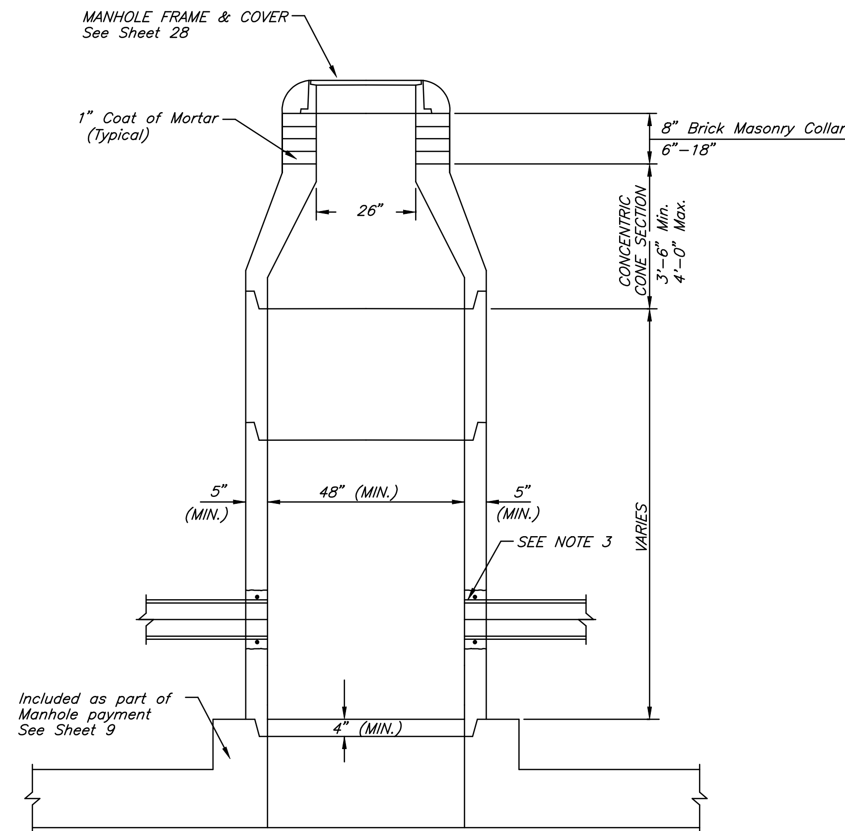
TYPICAL RCB MANHOLE
