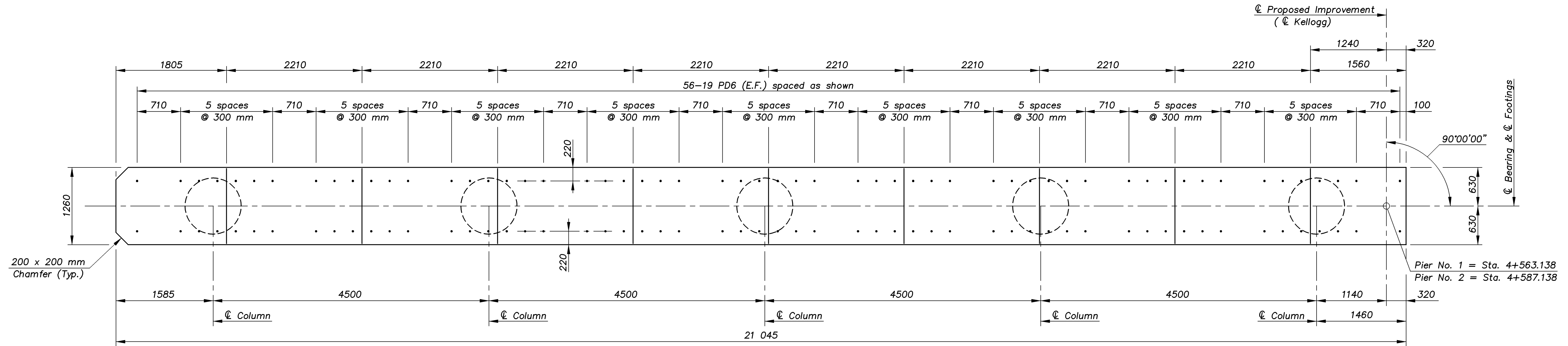
PLAN VIEW TOP OF PIER BEAM
