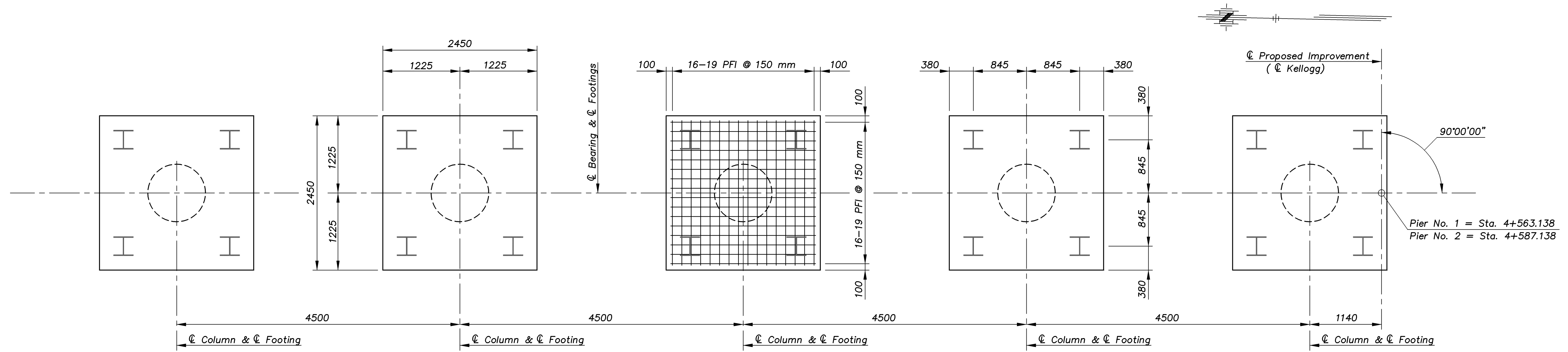
FOOTING LAYOUT
