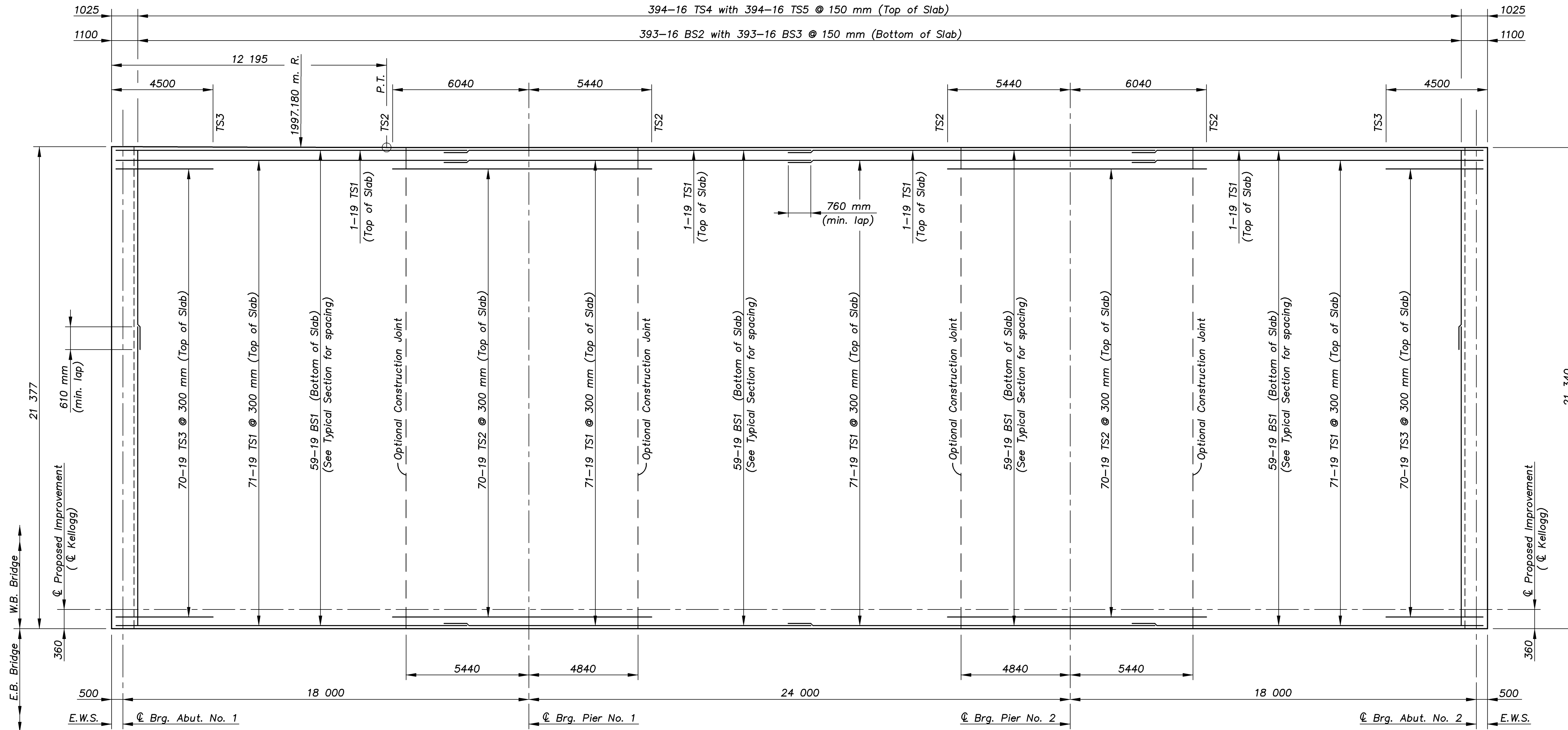
SLAB REINFORCEMENT PLAN
