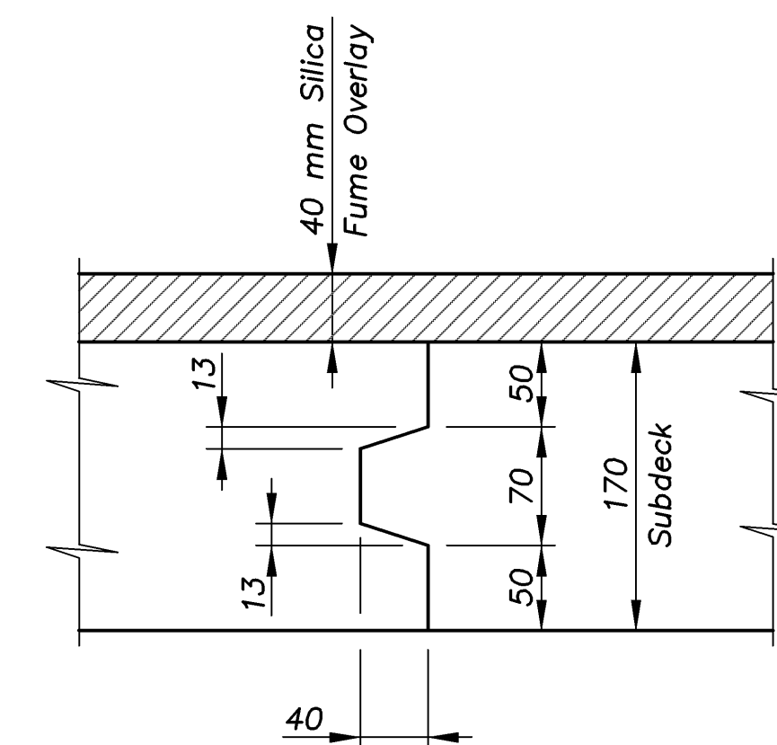
OPTIONAL CONSTRUCTION JOINT
