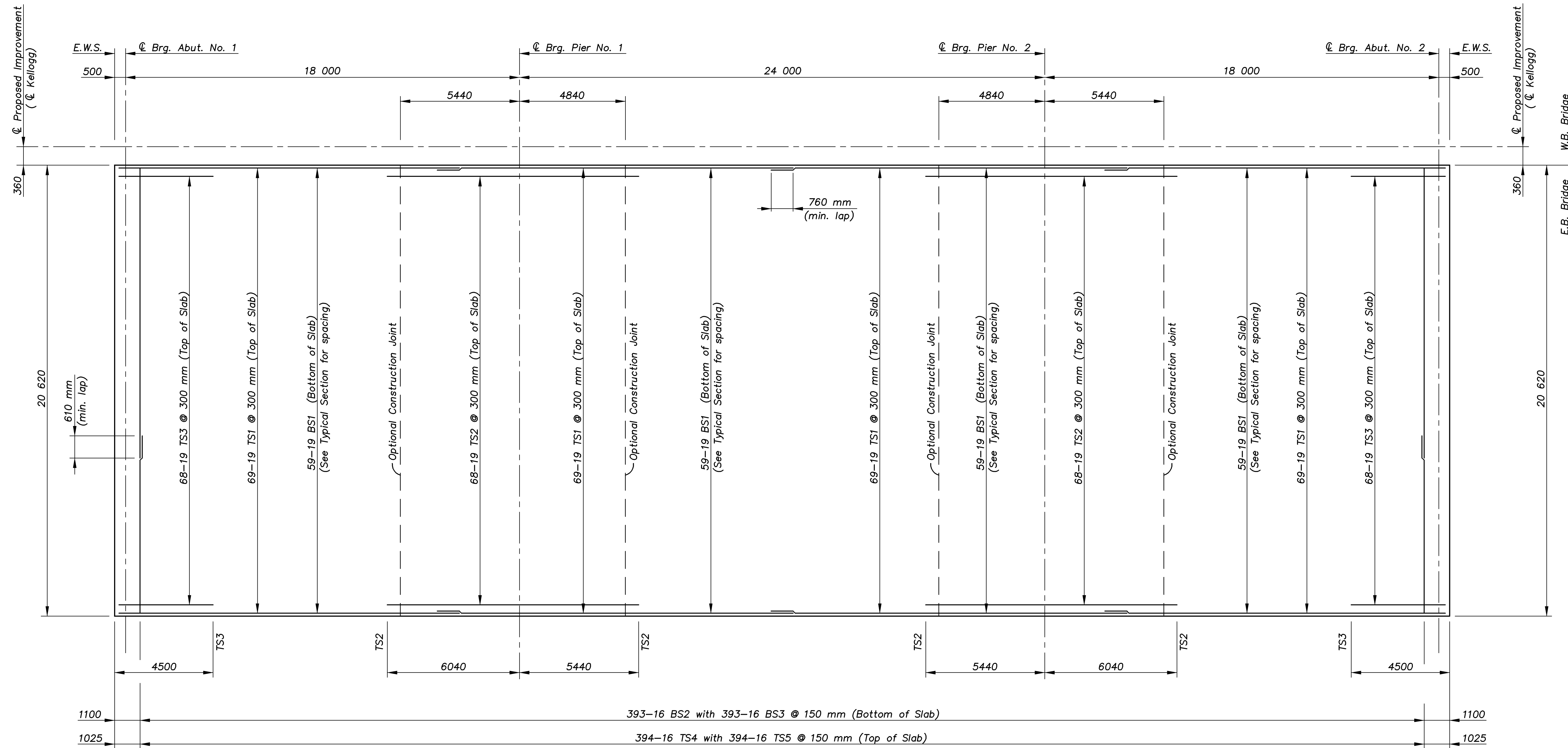
SLAB REINFORCEMENT PLAN
