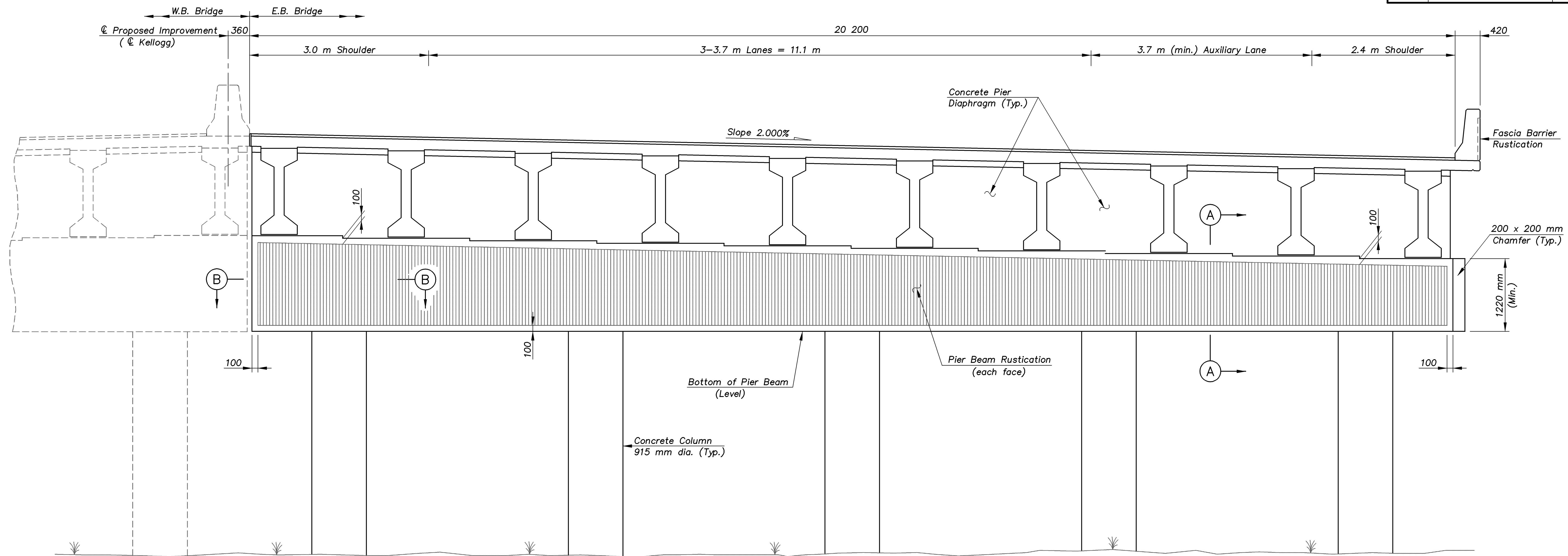
TYPICAL ELEVATION VIEW OF PIER (E.B. Bridge shown, W.B. Bridge similar)
