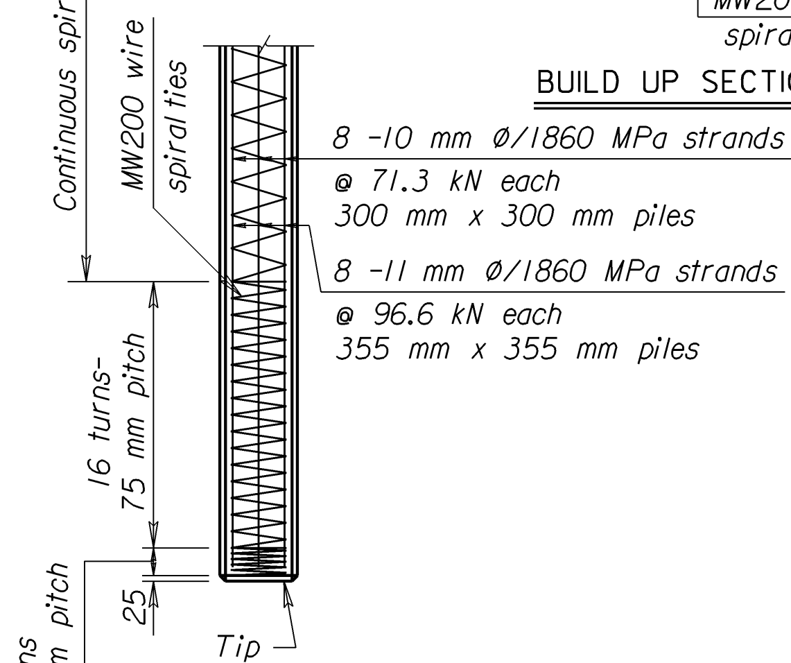
300 mm OR 355 mm PRESTRESSED CONCRETE PILES
