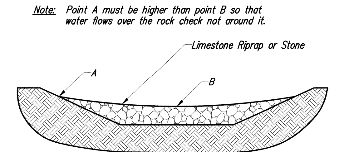
INSTALLATION OF ROCK DITCH CHECKS
