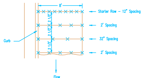
STAPLE PATTERN NOTES: Use 6" seam overlap
