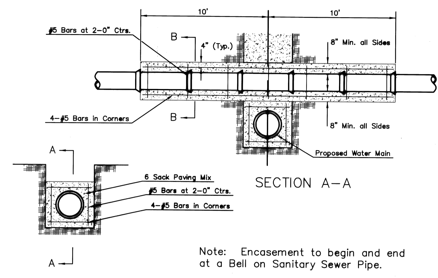
SECTION A-A SECTION B-B REINFORCED CONCRETE ENCASEMENT OF SANITARY SEWER
