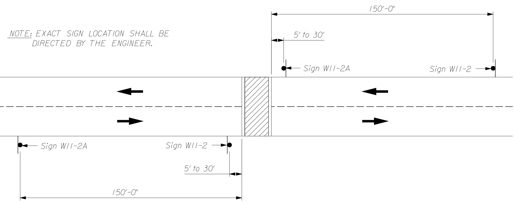
CROSSWALK SIGN SCHEMATIC NTS
