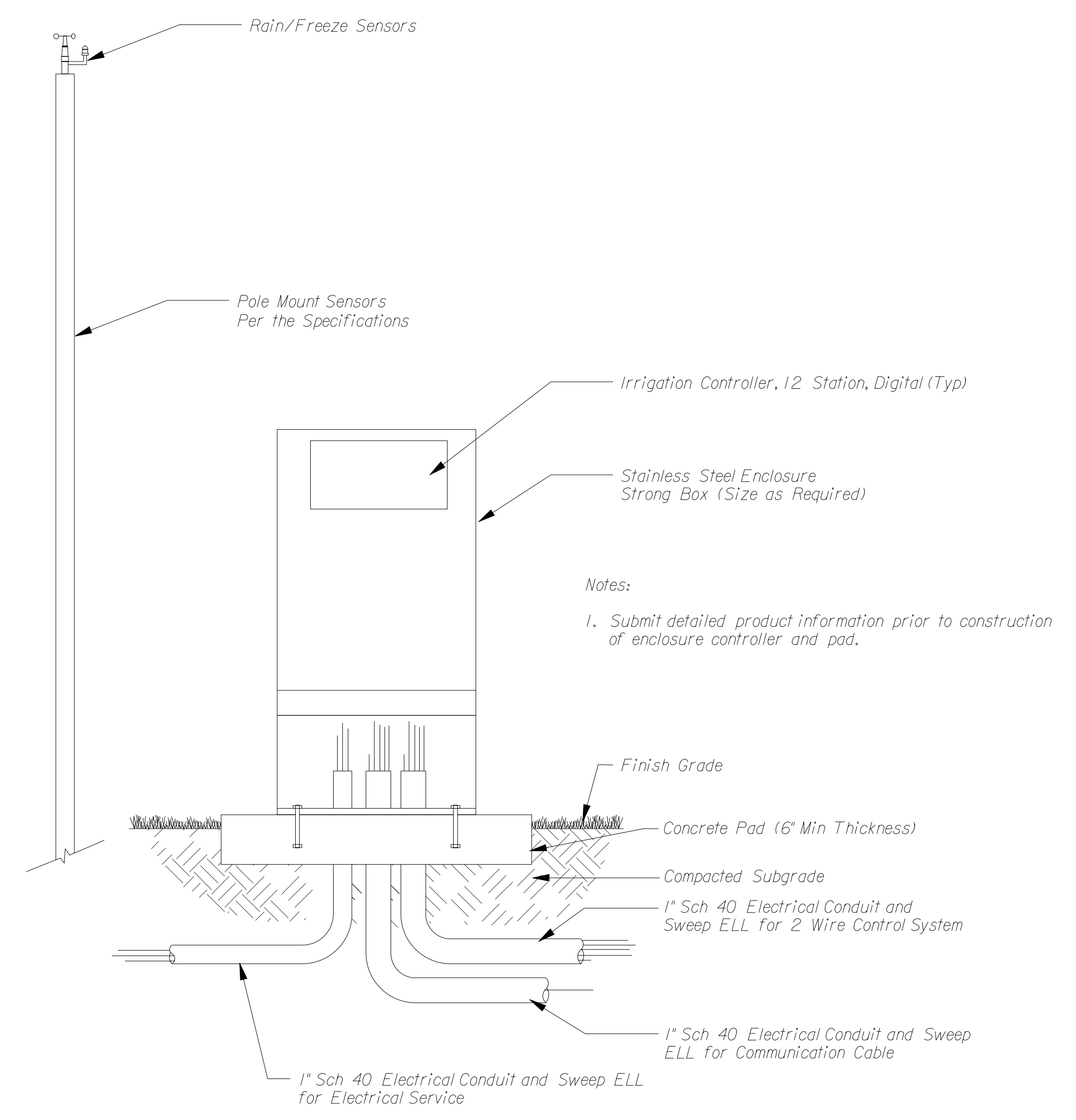
02 Front Elevation/Section - Controller NTS
