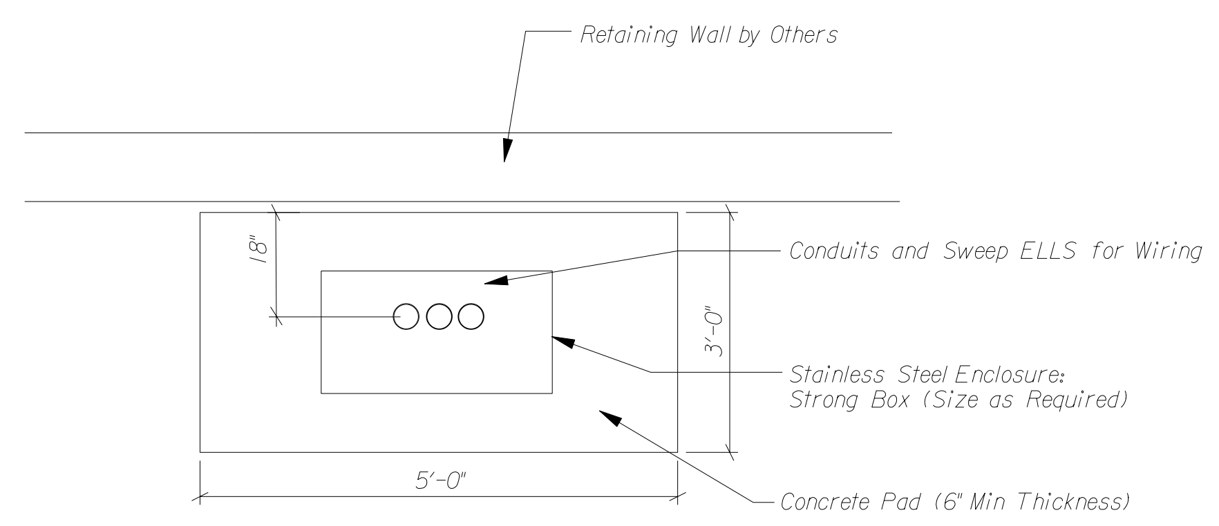
02 Front Elevation/Section LS3.15
