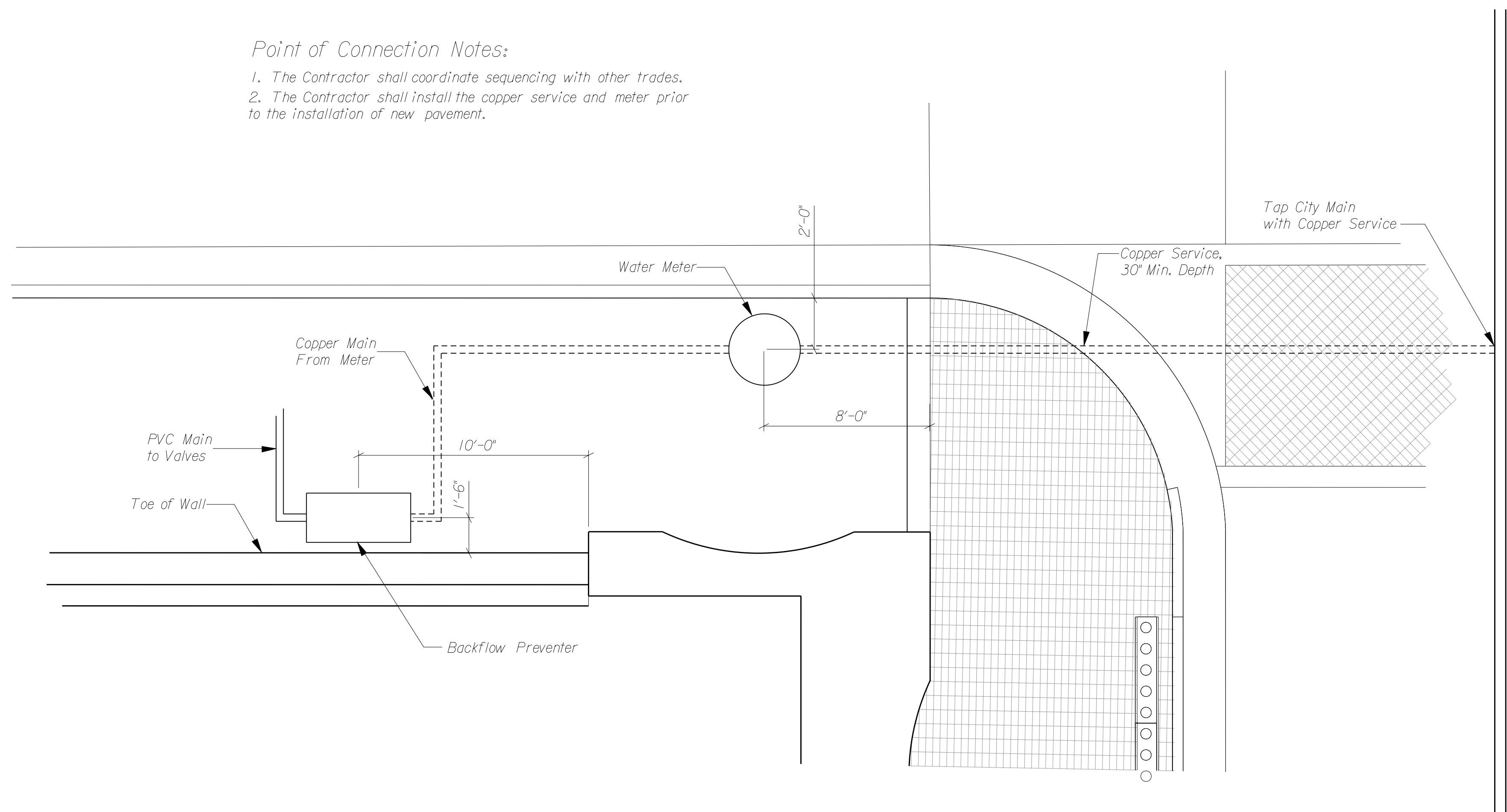
02 POINT OF CONNECTION SCHEMATIC NTS
