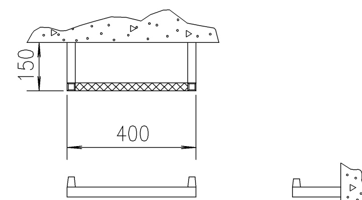
STEP DETAILS
