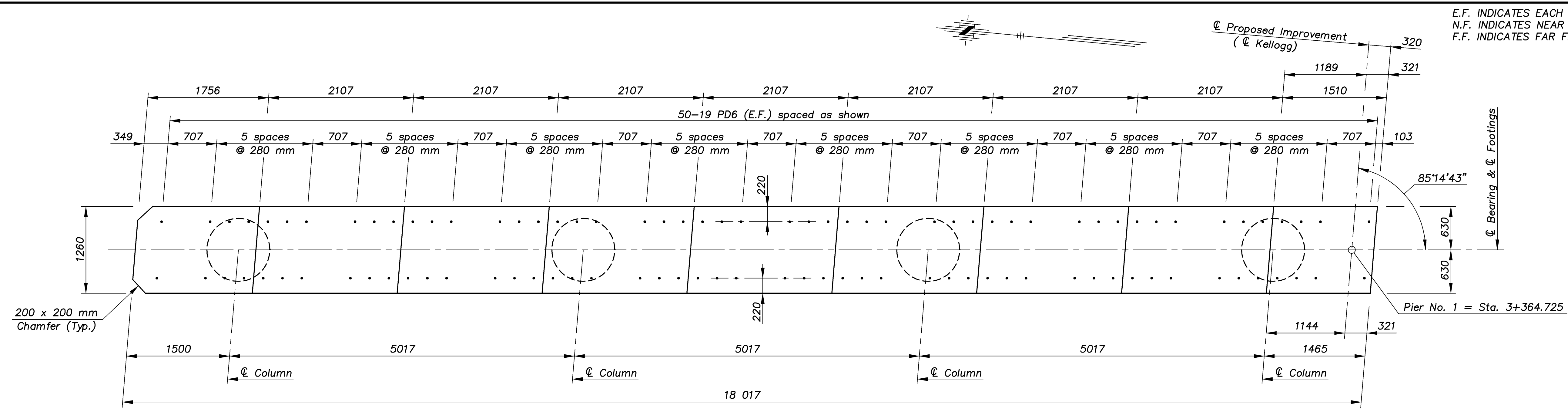
PLAN VIEW TOP OF PIER BEAM
