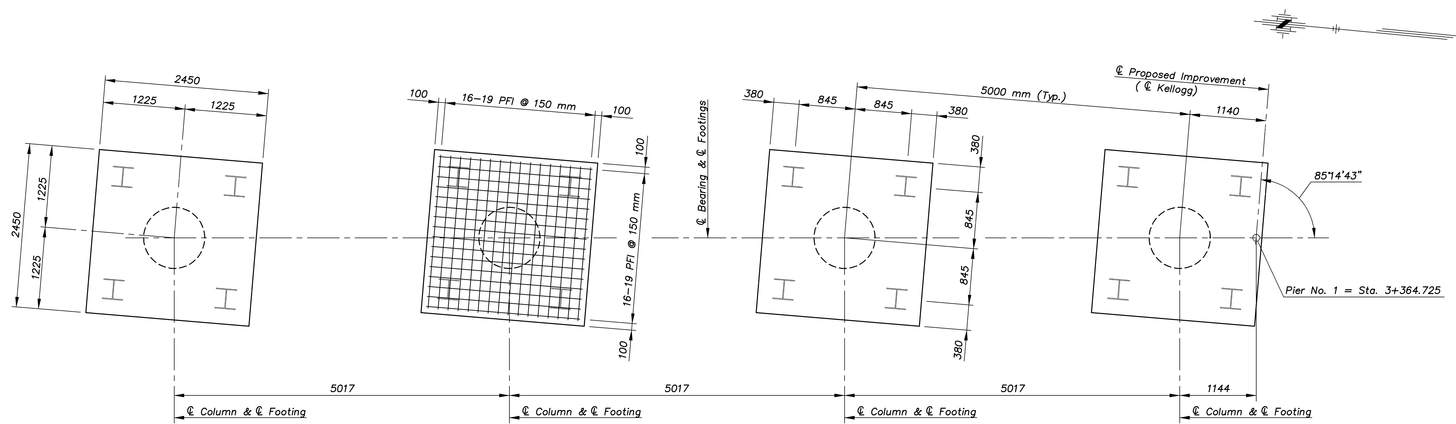
FOOTING LAYOUT
