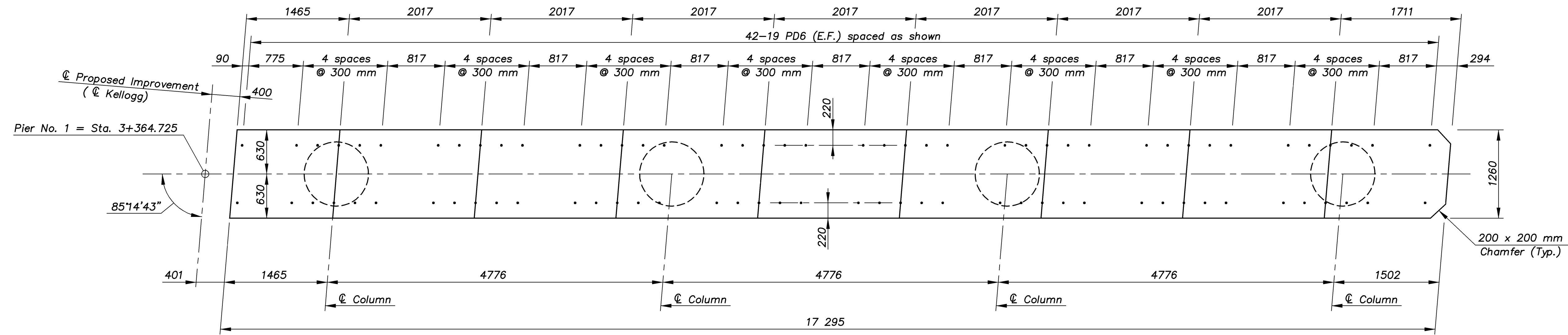
PLAN VIEW TOP OF PIER BEAM
