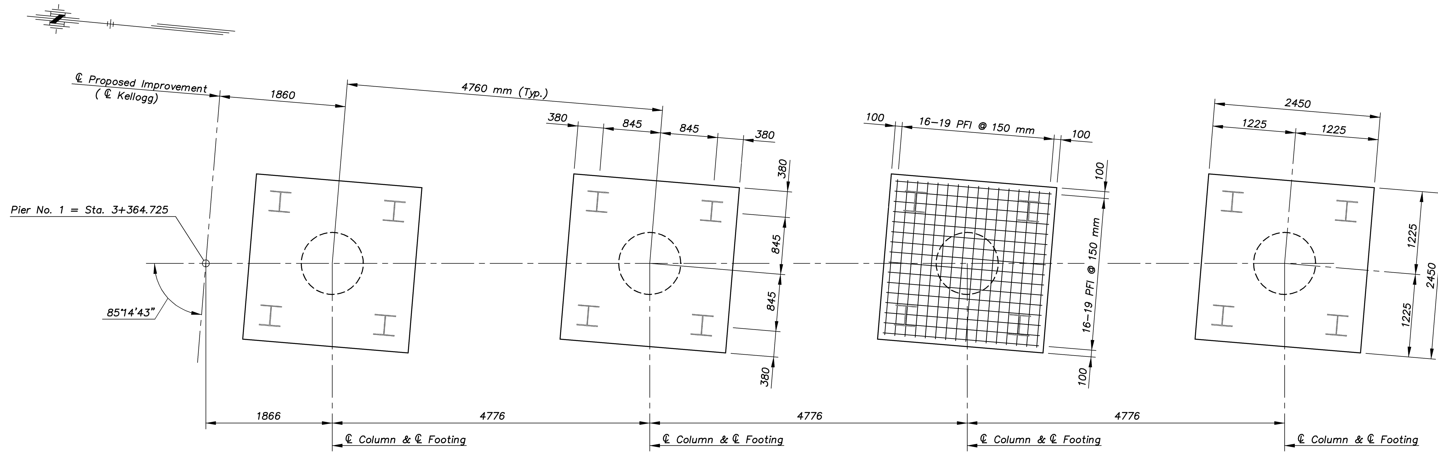
FOOTING LAYOUT
